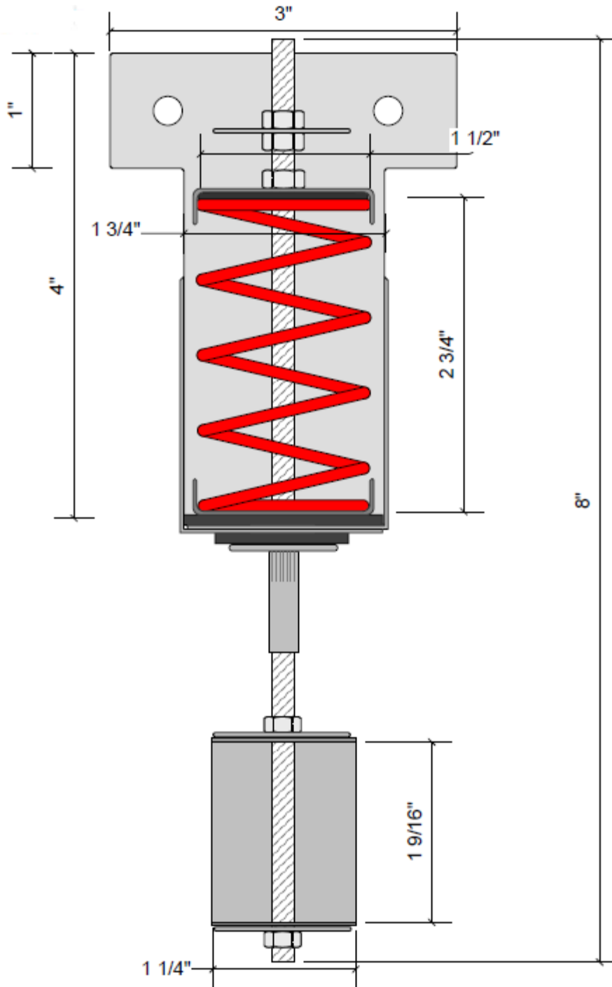
FRONT VIEW
