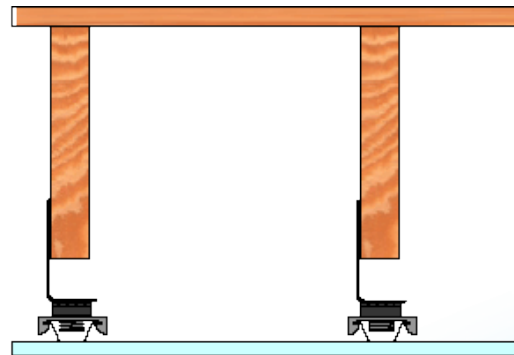
Dropped Ceiling Installation
